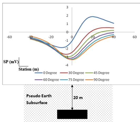
Figure 13: Superposition of SP Anomaly Curves for 20 m Depth of Burial at Different Dip.
