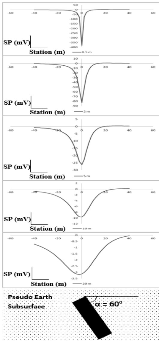
Figure 4: SP Profiles for 60° Geologic Dip.
