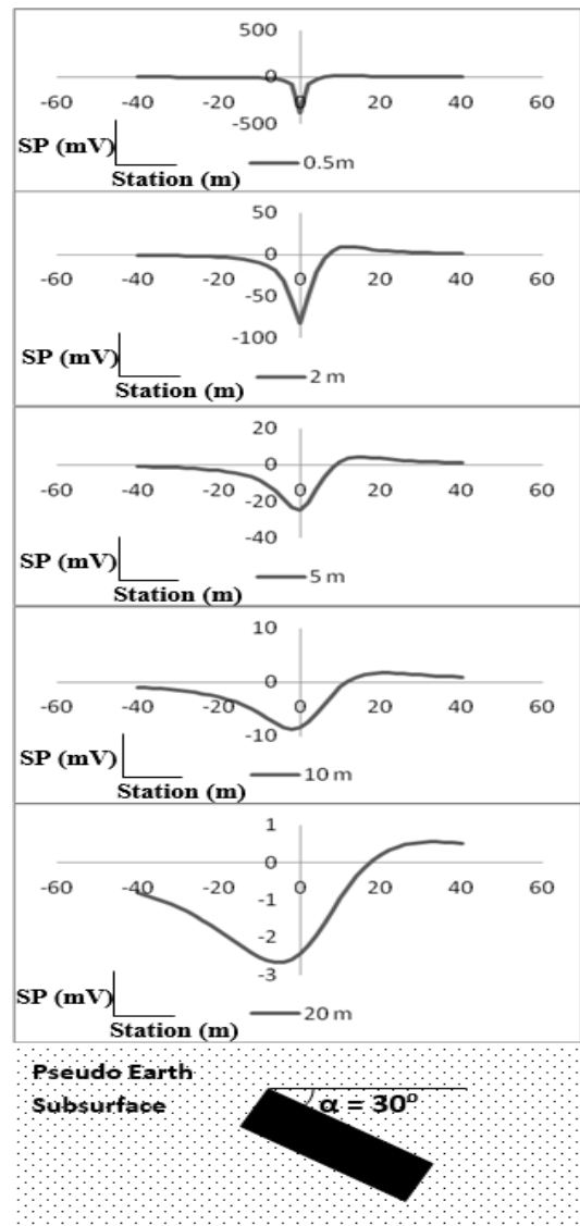
Figure 3: SP Profiles for 30° Geologic Dip.
