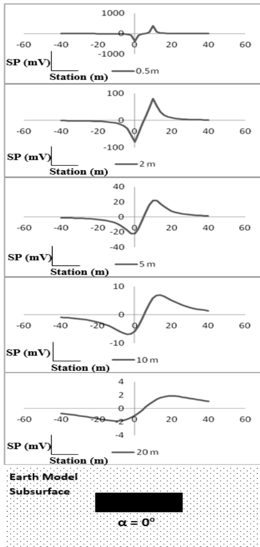
Figure 2: SP Profiles for 0° Geologic Dip.
