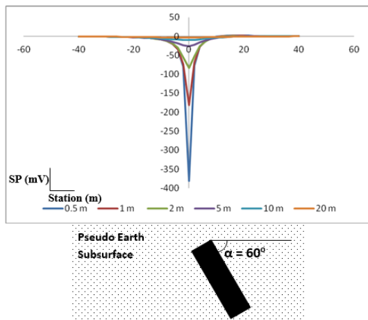
Figure 8: Superposition of SP Anomaly Curves for 60° at Different Depth of Burial.
