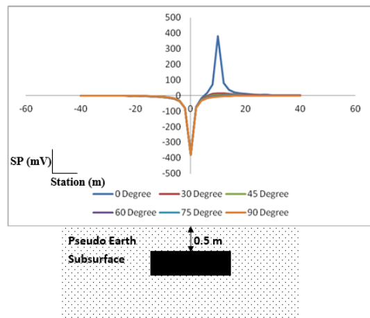
Figure 10: Superposition of SP Anomaly Curves for 0.5 m Depth of Burial at Different Dip.
