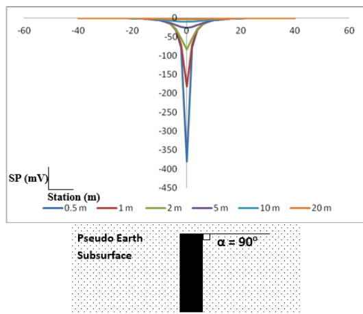
Figure 9: Superposition of SP Anomaly Curves for 90 at Different Depth of Burial.
