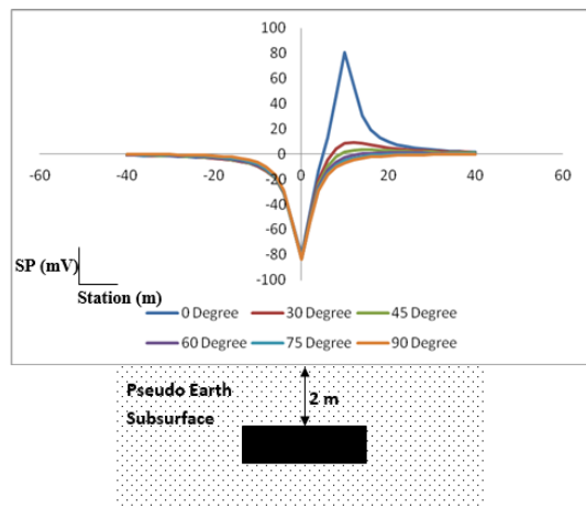
Figure 11: Superposition of SP Anomaly Curves for 2 m Depth of Burial at Different Dip.
