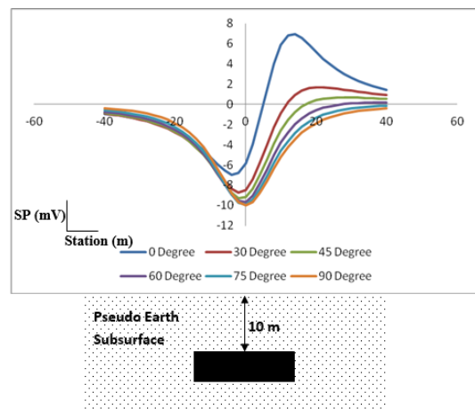
Figure 12: Superposition of SP Anomaly Curves for 10 m Depth of Burial at Different Dip.
