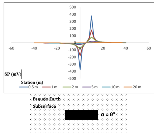
Figure 6: Superposition of SP Anomaly Curves for 0^\circ at Different Depth of Burial.
