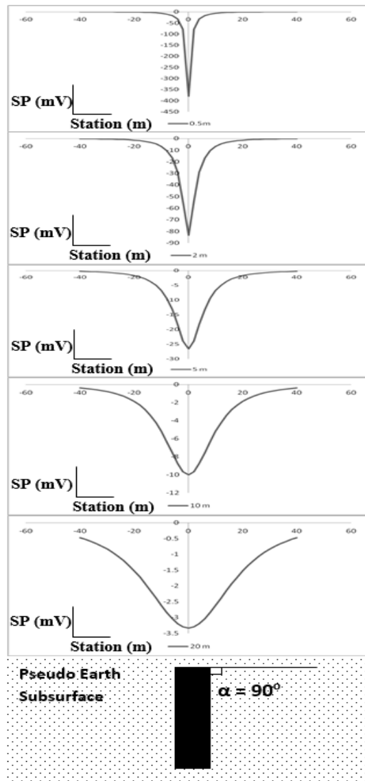
Figure 5: SP Profiles for 90° Geologic Dip.
