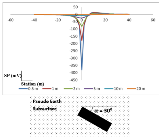
Figure 7: Superposition of SP Anomaly Curves for 30° at Different Depth of Burial.
