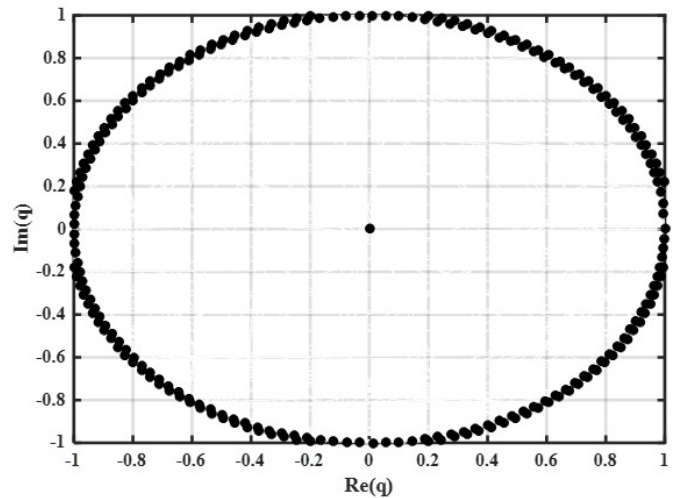
Figure 1. Absolute stability region of proposed method
