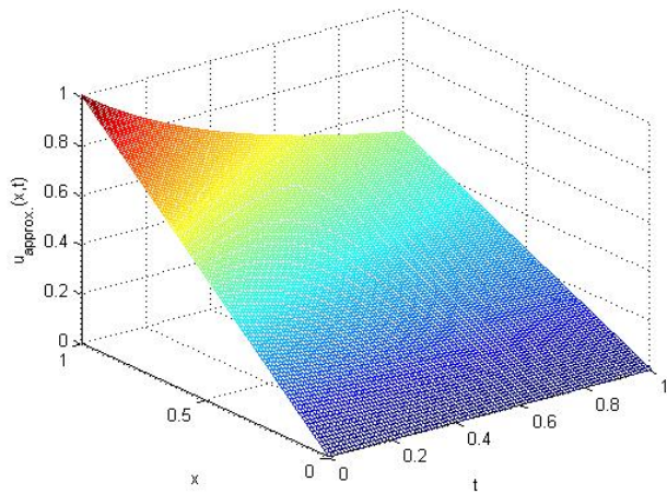
Figure 8: Graph of Exact Solution of Example 3
