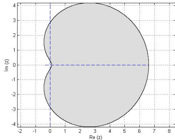
Figure 2: Stability Region of Method (33)
