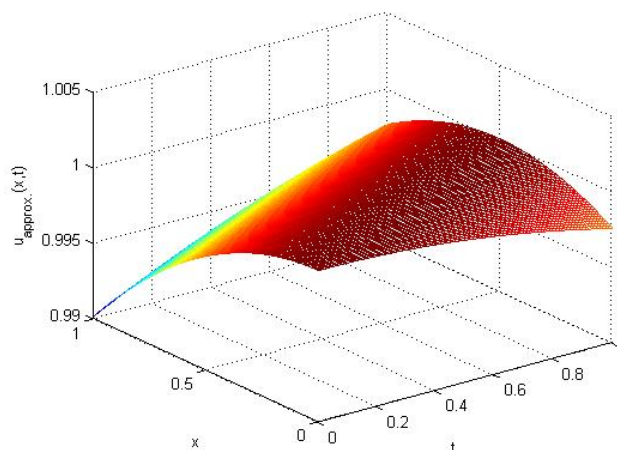
Figure 5: Graph of Numerical Solution of Example 1
