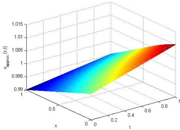
Figure 7: Graph of Numerical Solution of Example 2
