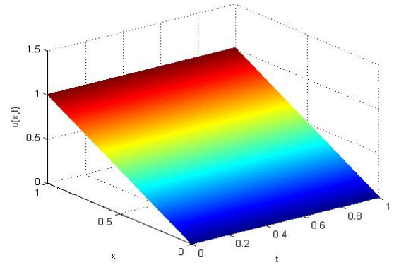
Figure 10: Graph of Exact Solution of Example 4
