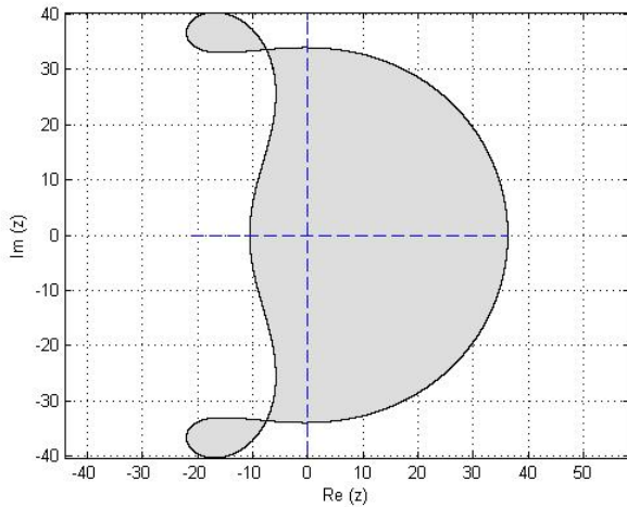
Figure 3: Stability Region of Method (40)
