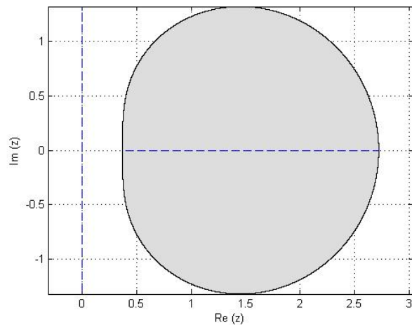
Figure 1: Stability Region of Method (27)
