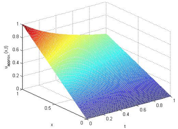
Figure 9: Graph of Numerical Solution of Example 3
