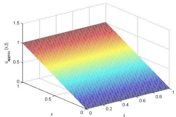
Figure 11: Graph of Numerical Solution of Example 4
