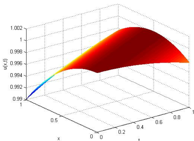
Figure 4: Graph of Exact Solution of Example 1
