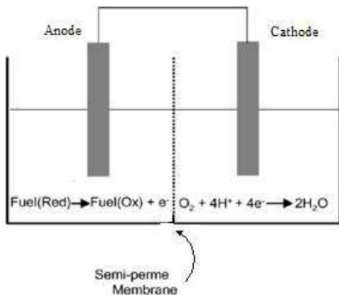
Figure 1: Working principle of a fuel cell [4].
