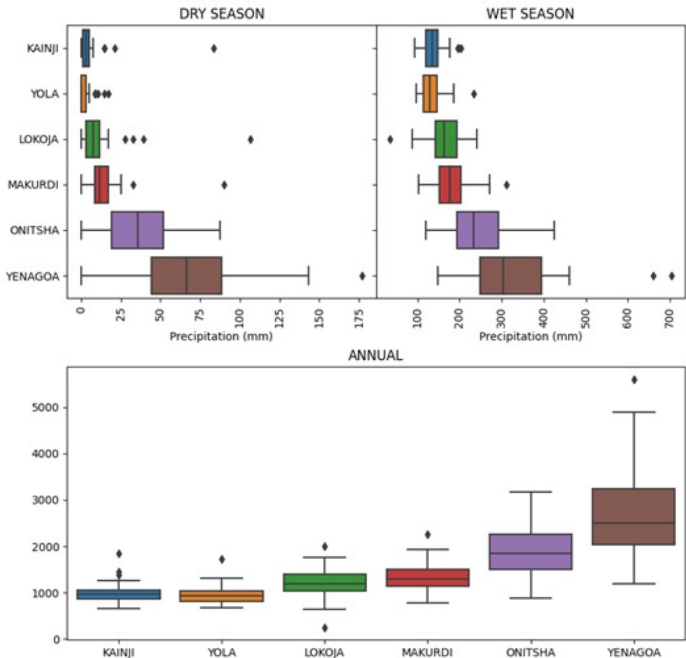
Figure 5. Box plots showing the data distribution for dry season, wet season, and the annual trend across all years for all study locations.
