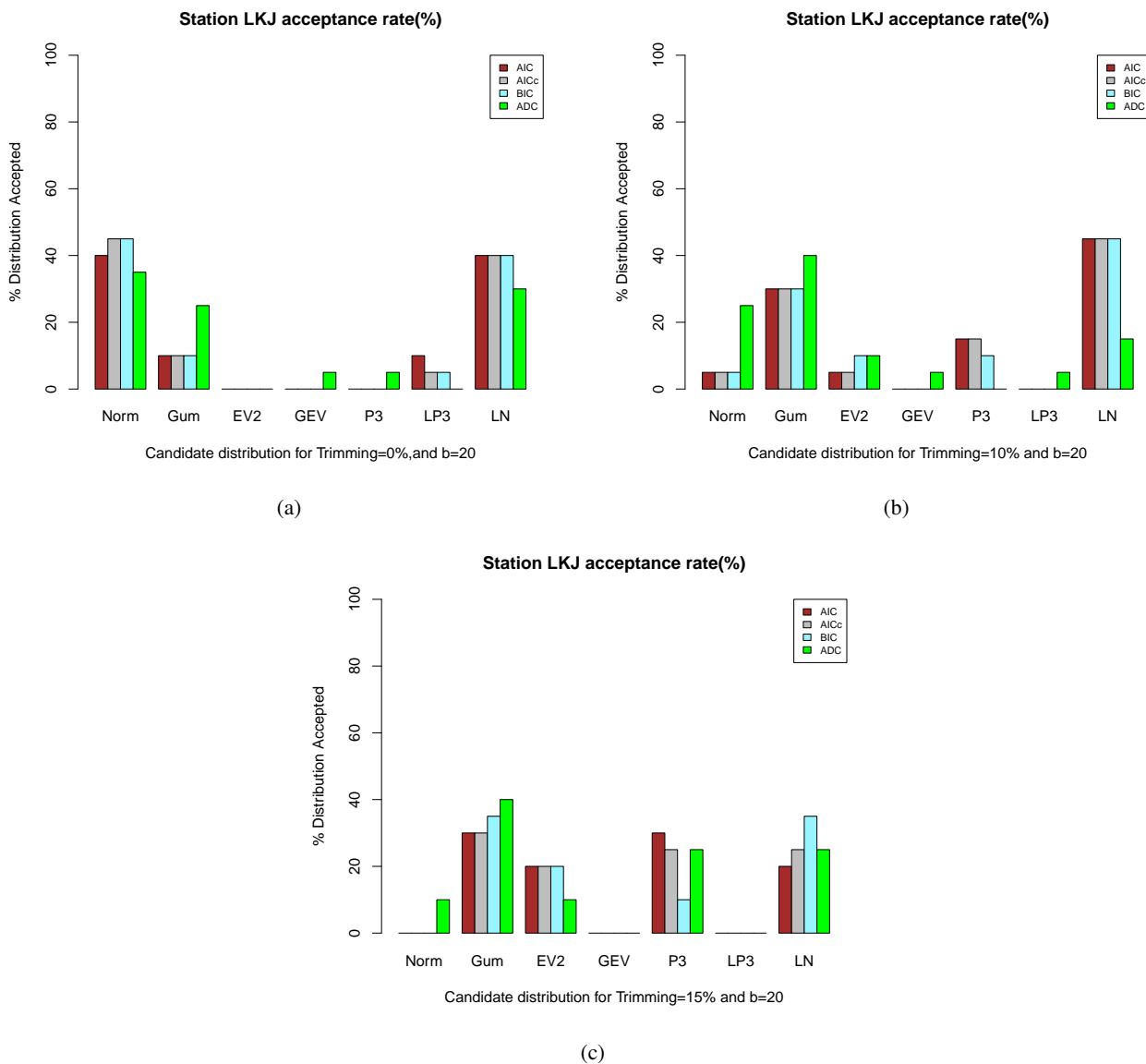
Figure 14: Percentage of cases a candidate distribution is accepted for subsample size 20.
