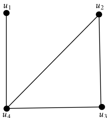
Figure 3: Graph \Theta_2^* = (\varpi_2, \tau_2) .
