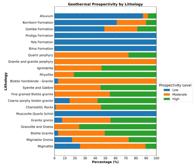
Figure 14. Stacked bar chart of geothermal prospectivity distribution across lithological units (by percentage).
