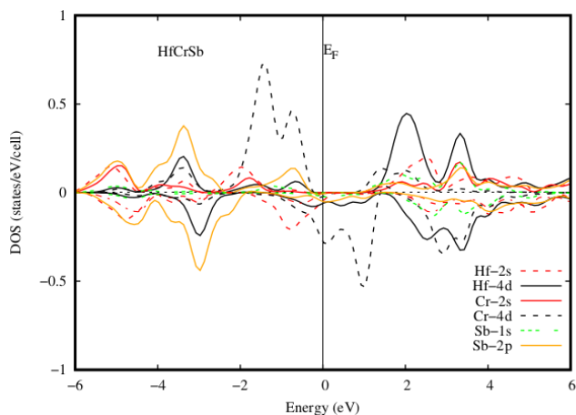
Figure 9. PDOS for HfCrSb alloy
