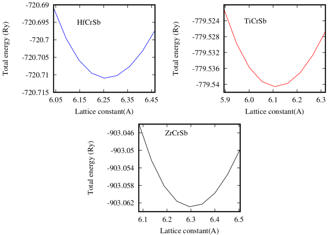
Figure 2. Relationship between total energies per unit cell and lattice parameters for HfCrSb, TiCrSb and ZrCrSb
