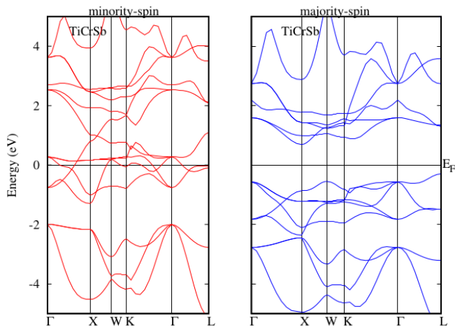
Figure 4. Band structure of TiCrSb alloy
