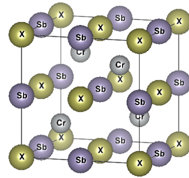
Figure 1. The crystal structure of XCrSb where X = Ti, Zr and Hf.
