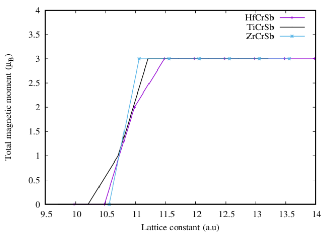
Figure 10. Total magnetic moment per formula unit as a function of lattice constants for the three alloys.
