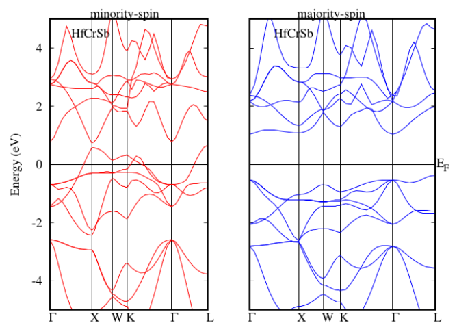
Figure 6. Band structure of HfCrSb alloy
