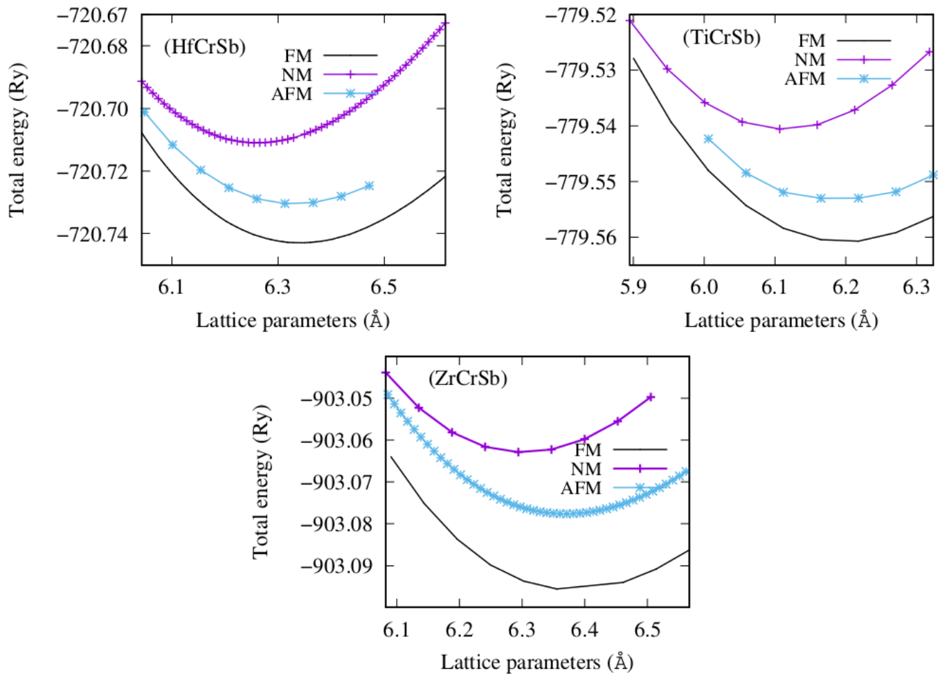
Figure 3. The total energies per unit cell as a function of lattice constants for the Ferromagnetic (FM), Antiferromagnetic (AFM) and Non-magnetic (NM) states of the alloys.
