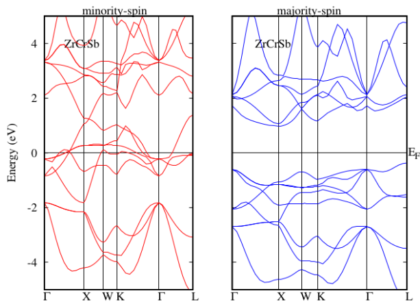
Figure 5. Band structure of ZrCrSb alloy
