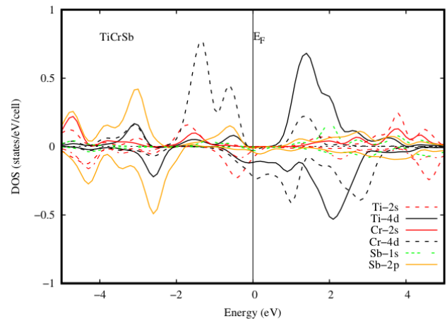
Figure 7. PDOS for TiCrSb alloy
