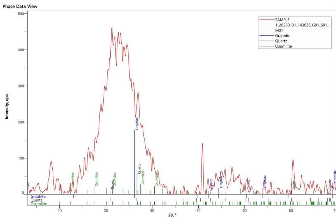
Figure S1: XRD pattern of rice husk biochar
