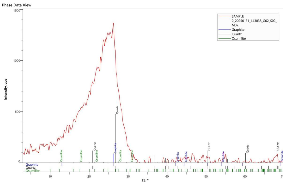
Figure S2: XRD pattern of cow horn biochar
