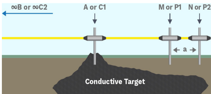
Figure 11: Mise-A-La-Masse array (modified from Advanced Geoscience, Inc).
