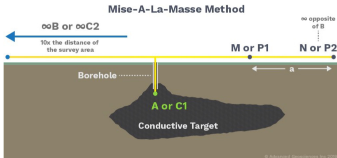
Figure 12: Mise-A-La-Masse array (modified from Advanced Geoscience, Inc).
