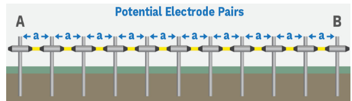
Figure 9: Gradient array (modified from Advanced Geoscience, Inc).
