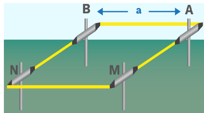
Figure 7: Square array (modified from Advanced Geoscience, Inc).
