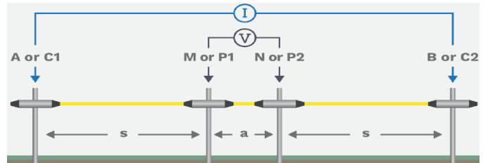
Figure 2: Schlumberger array (modified from Advanced Geoscience, Inc).
