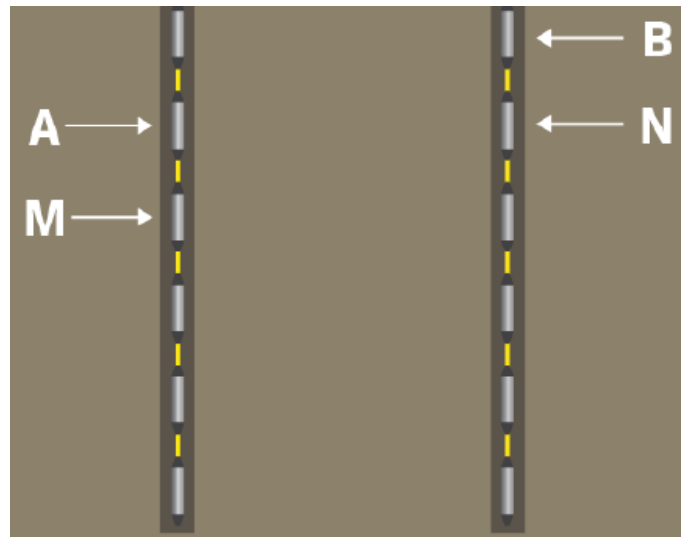
Figure 13: Bipole-Bipole array (modified from Advanced Geoscience, Inc).
