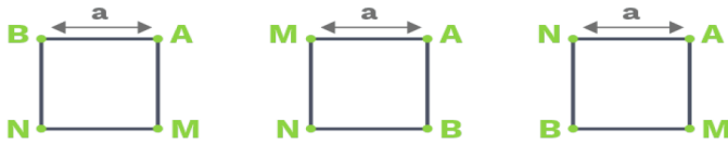
Figure 8: Square array (modified from Advanced Geoscience, Inc).
