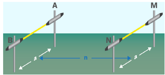
Figure 6: Equatorial array (modified from Advanced Geoscience, Inc).
