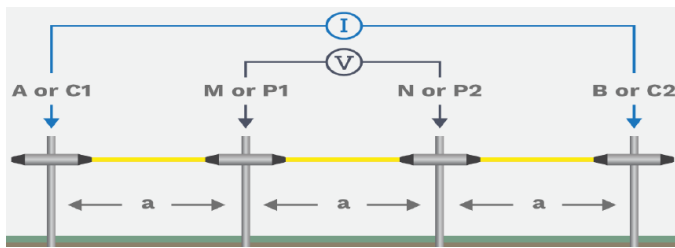
Figure 1: Wenner array (modified from Advanced Geoscience, Inc).
