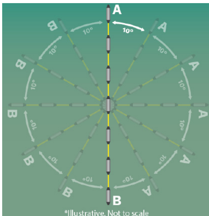
Figure 10: Azimuthal Method (modified from Advanced Geoscience, Inc).
