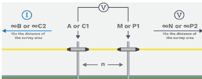
Figure 5: Pole-Pole array (modified from Advanced Geoscience, Inc).
