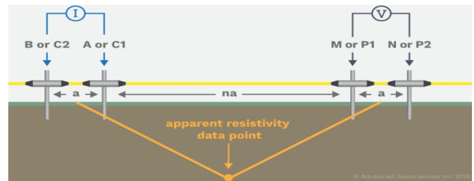
Figure 3: Dipole-Dipole array (modified from Advanced Geoscience, Inc).
