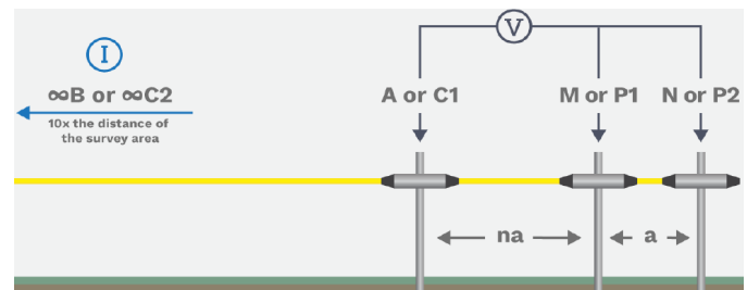
Figure 4: Pole-Dipole array (modified from Advanced Geoscience, Inc).
