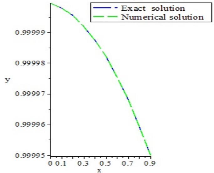
Figure 1: Comparison of the exact and numerical solutions for example 1.
