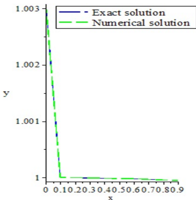
Figure 2: Comparison of the exact and numerical solutions for example 2.
