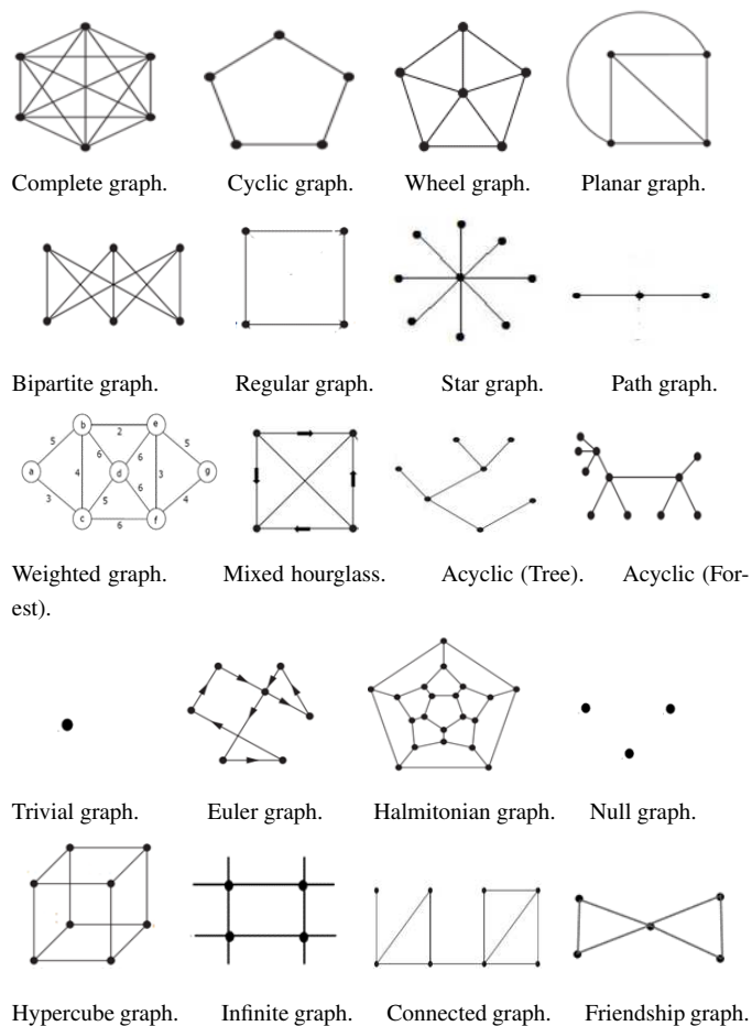
Figure 8. Basic graph types.
