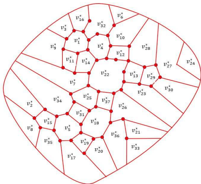
Figure 10. The Voronoi diagram of Nigeria map.
