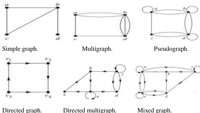
Figure 7. Graph classification.
