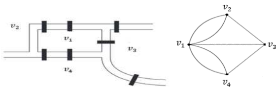
Figure 2. A graph representation of the bridges of Königsberg.
