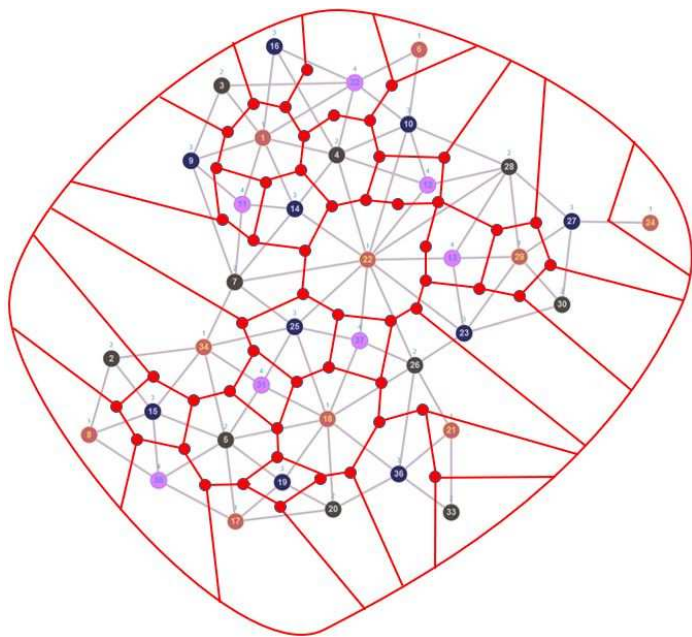
Figure 11. The dual graph of Nigeria map.
