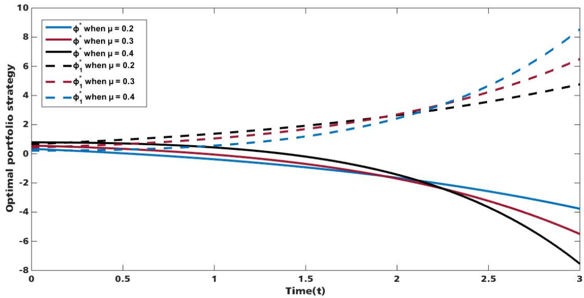
Figure 3. Time evolution of optimal portfolio strategy with different \mu .
