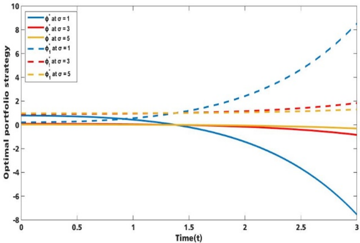
Figure 4. Time evolution of optimal portfolio strategy with different \sigma .
