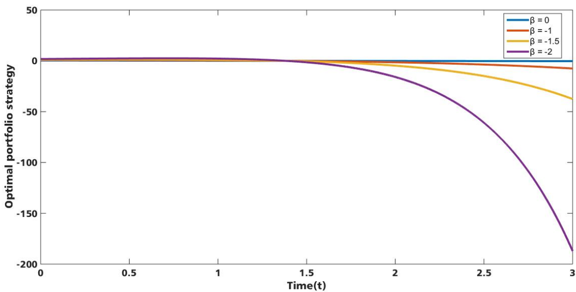
Figure 2. Time evolution of optimal portfolio strategy with different \beta .
