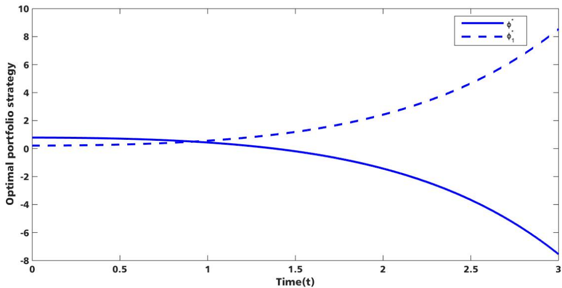
Figure 1. Time evolution of optimal portfolio strategies.
