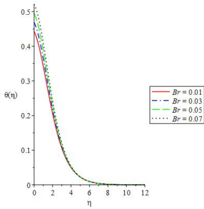
Figure 5. Heat profile for variation of Br
