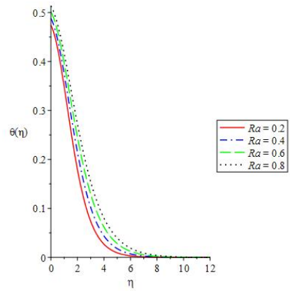
Figure 8. Rising Ra effect on temperature
