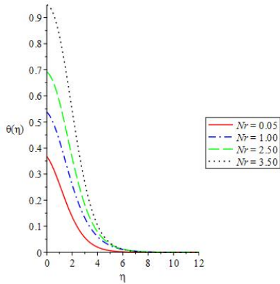
Figure 6. Plot of \theta(\eta) versus \eta for Nr
