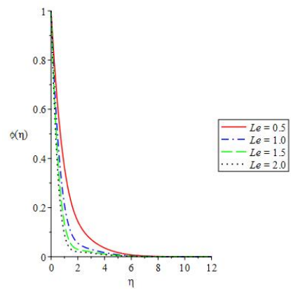
Figure 9. Reaction field for rising Le
