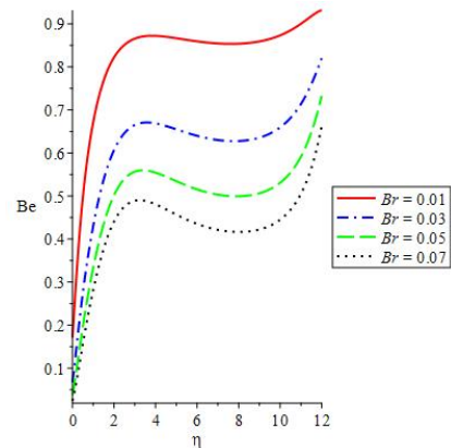
Figure 17. Irreversibility ratio field for Br
