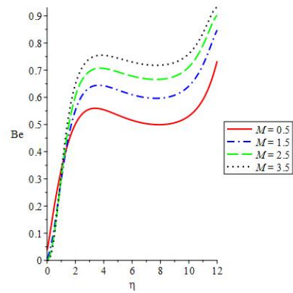
Figure 16. M effects on Bejan number
