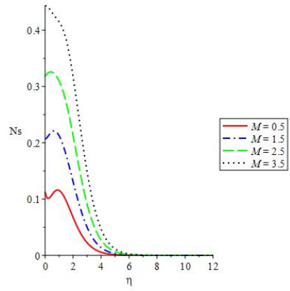
Figure 13. M impacts on entropy field
