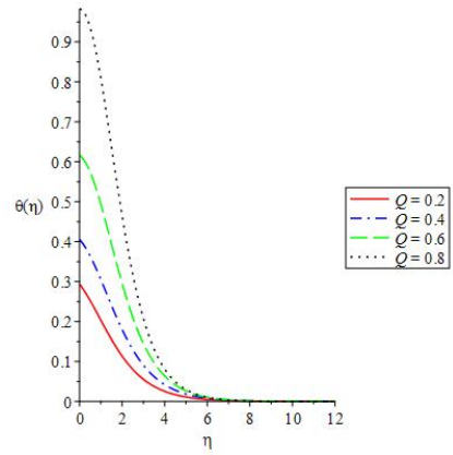
Figure 7. Temperature field for various Q
