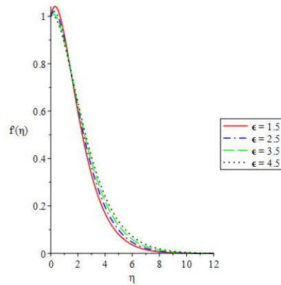
Figure 2. Flow rate field for various \epsilon
