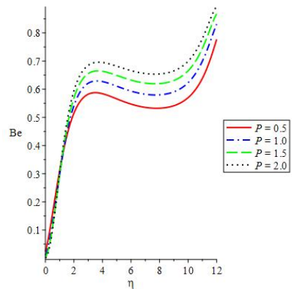
Figure 15. Impact of P on Bejan number
