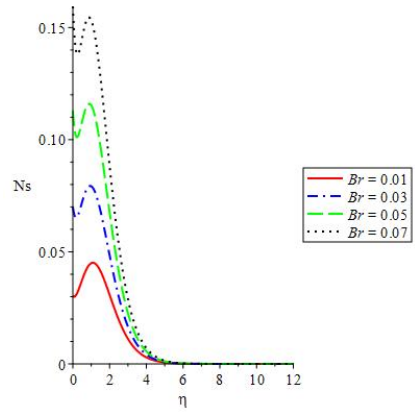
Figure 14. Irreversibility for increasing Br
