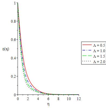
Figure 10. Effect of \Lambda on concentration
