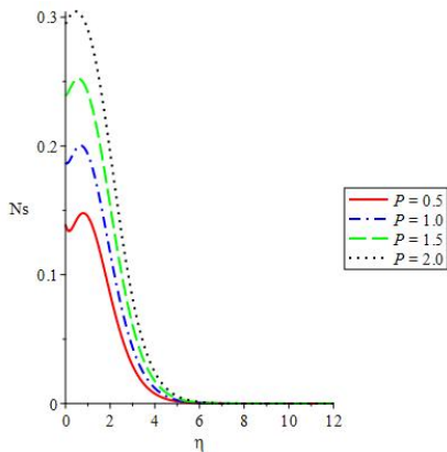
Figure 12. Entropy profile for different
