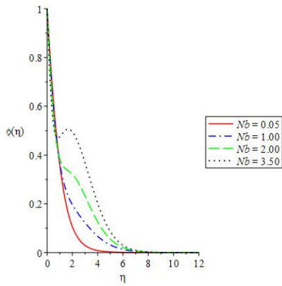
Figure 11. \phi(\eta) versus \eta for various Nb
