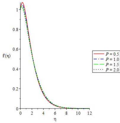
Figure 4. f(\eta) against \eta for various P
