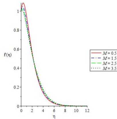
Figure 3. Velocity field for different M
